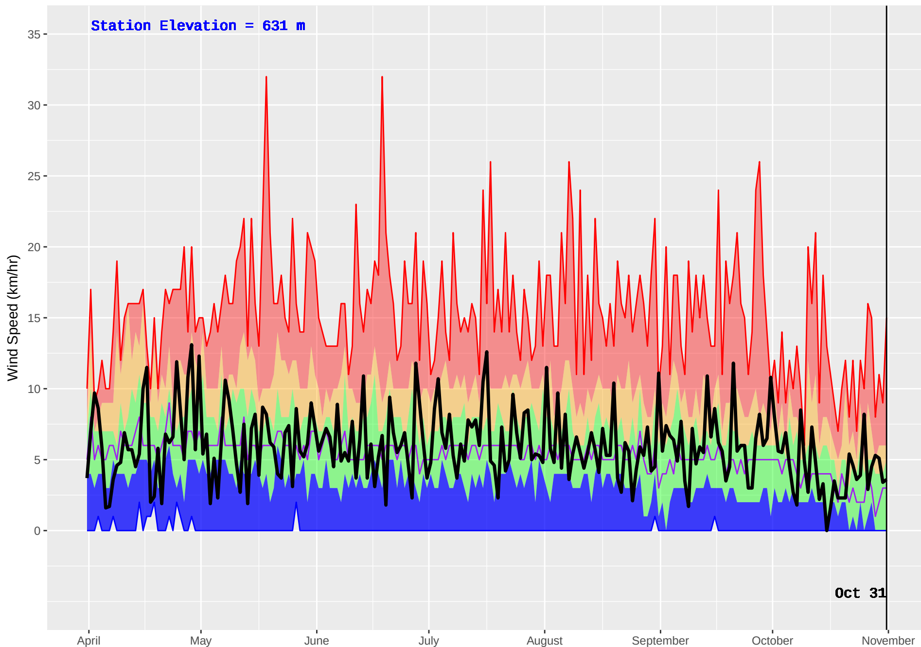
EAST BARRIERE (243) : Historical (1978–2016) and Current (2017) Noon Wind Speed
