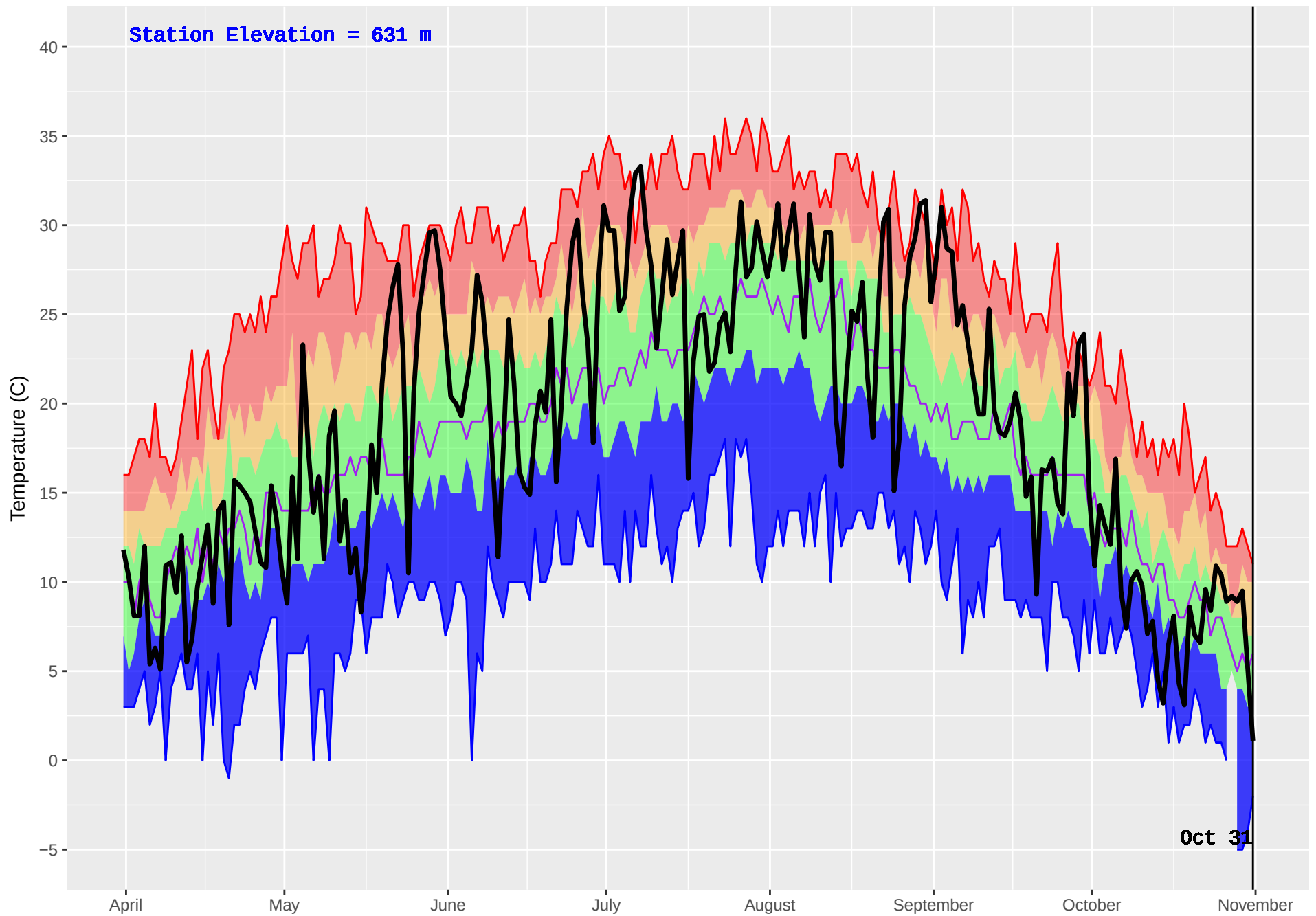
EAST BARRIERE (243) : Historical (1978–2016) and Current (2017) Noon Temperature
