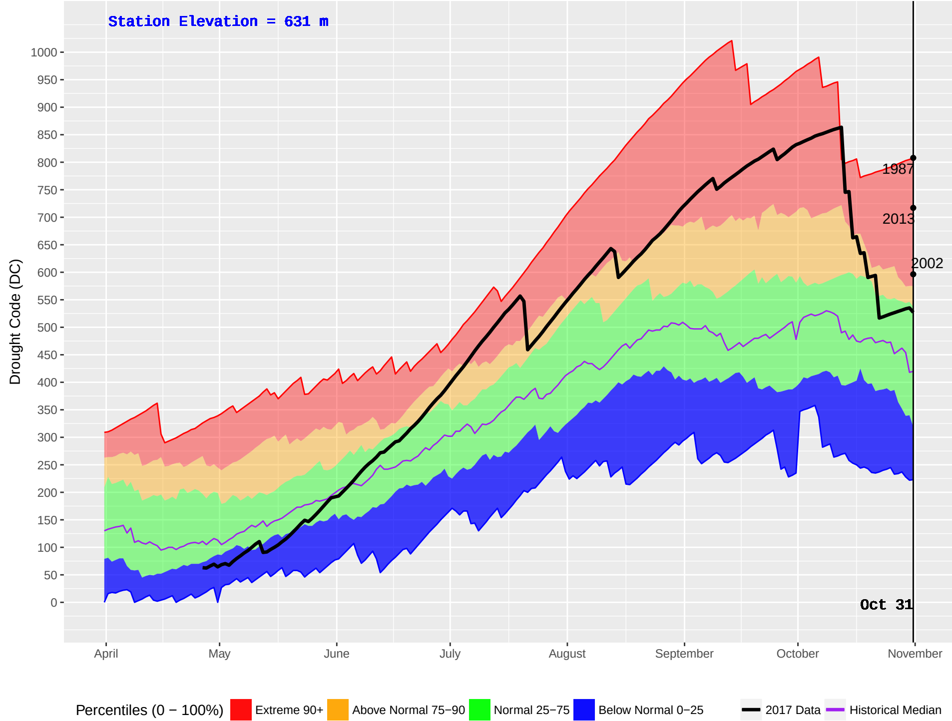
EAST BARRIERE (243) : Historical (1978–2016) and Current (2017) Noon Drought Code (DC)
