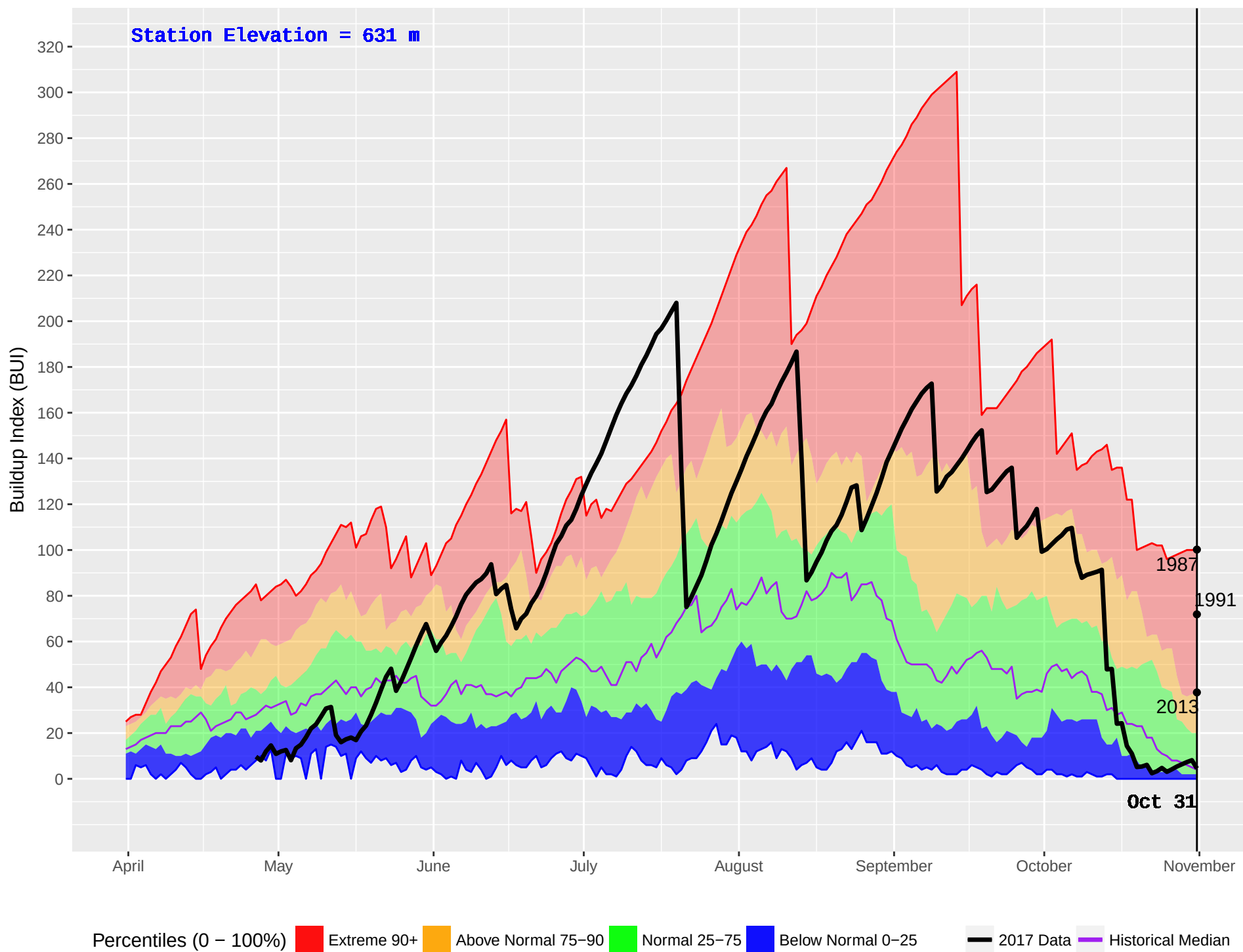
EAST BARRIERE (243) : Historical (1978–2016) and Current (2017) Noon Buildup Index (BUI)
