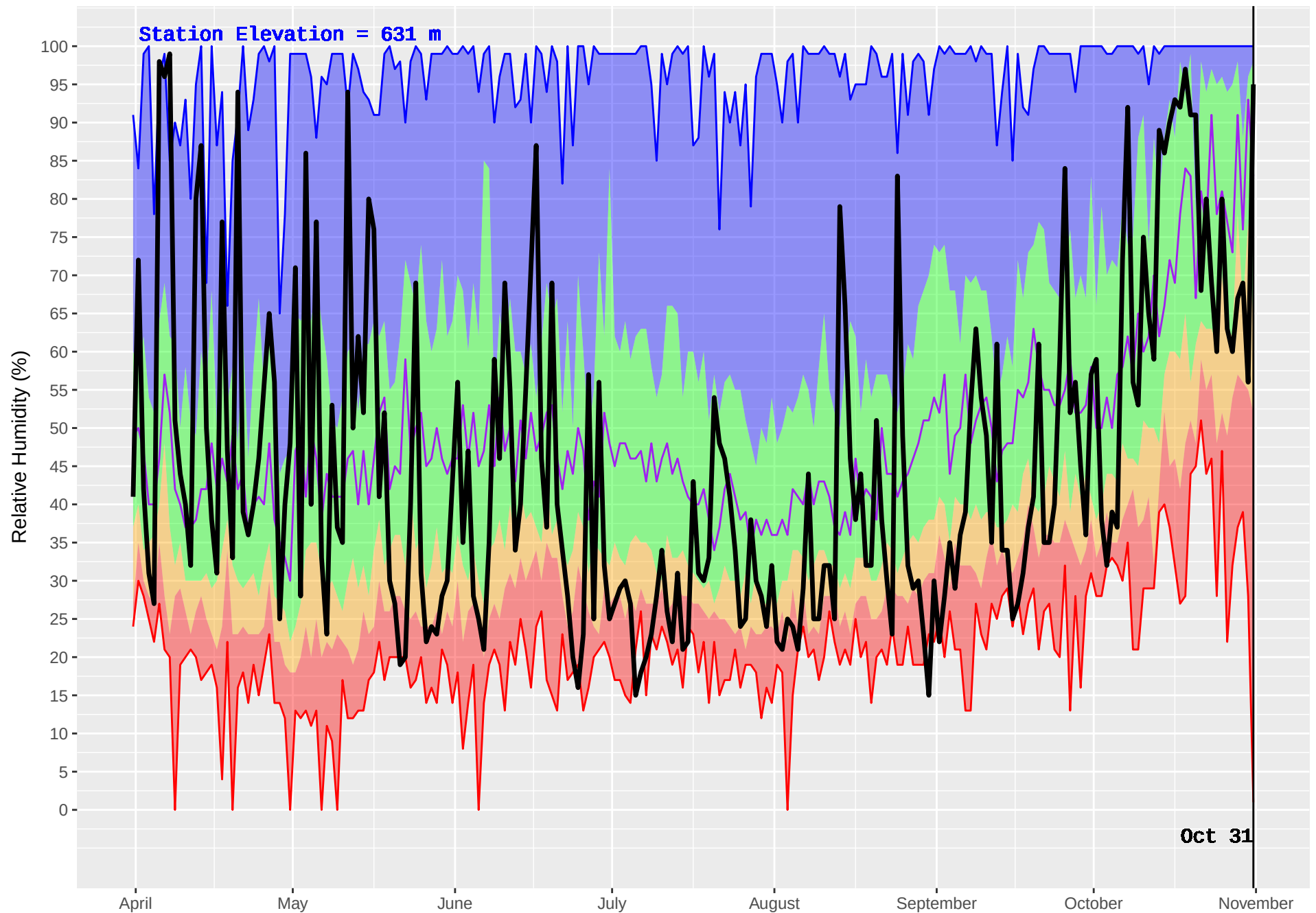
EAST BARRIERE (243) : Historical (1978–2016) and Current (2017) Noon Relative Humidity
