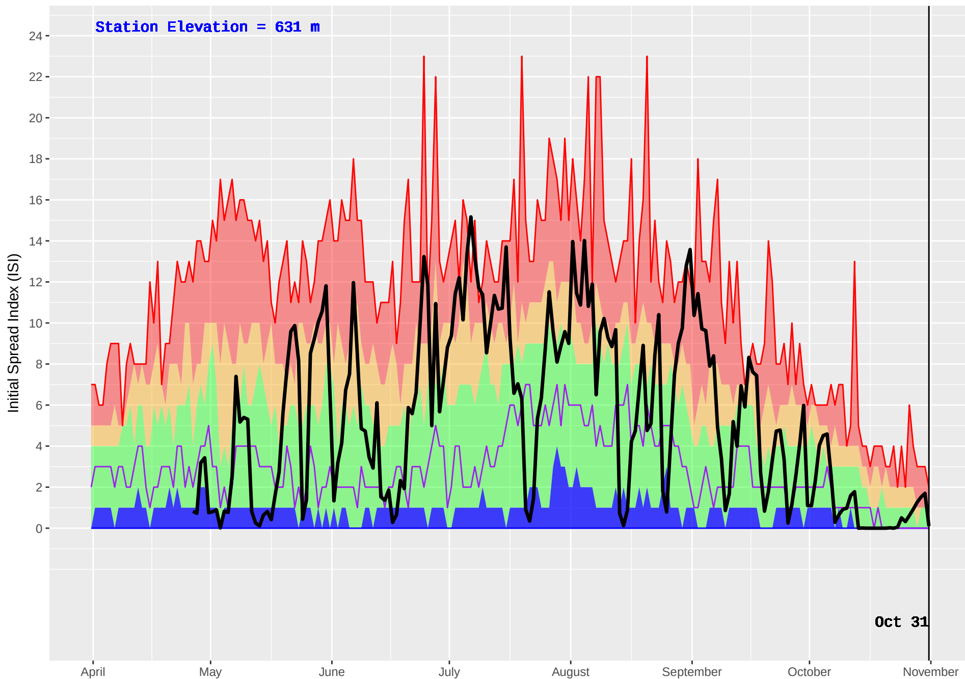
EAST BARRIERE (243) : Historical (1978–2016) and Current (2017) Noon Initial Spread Index (ISI)
